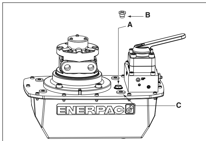
Figur 2, ZA4-ventilatormontering
