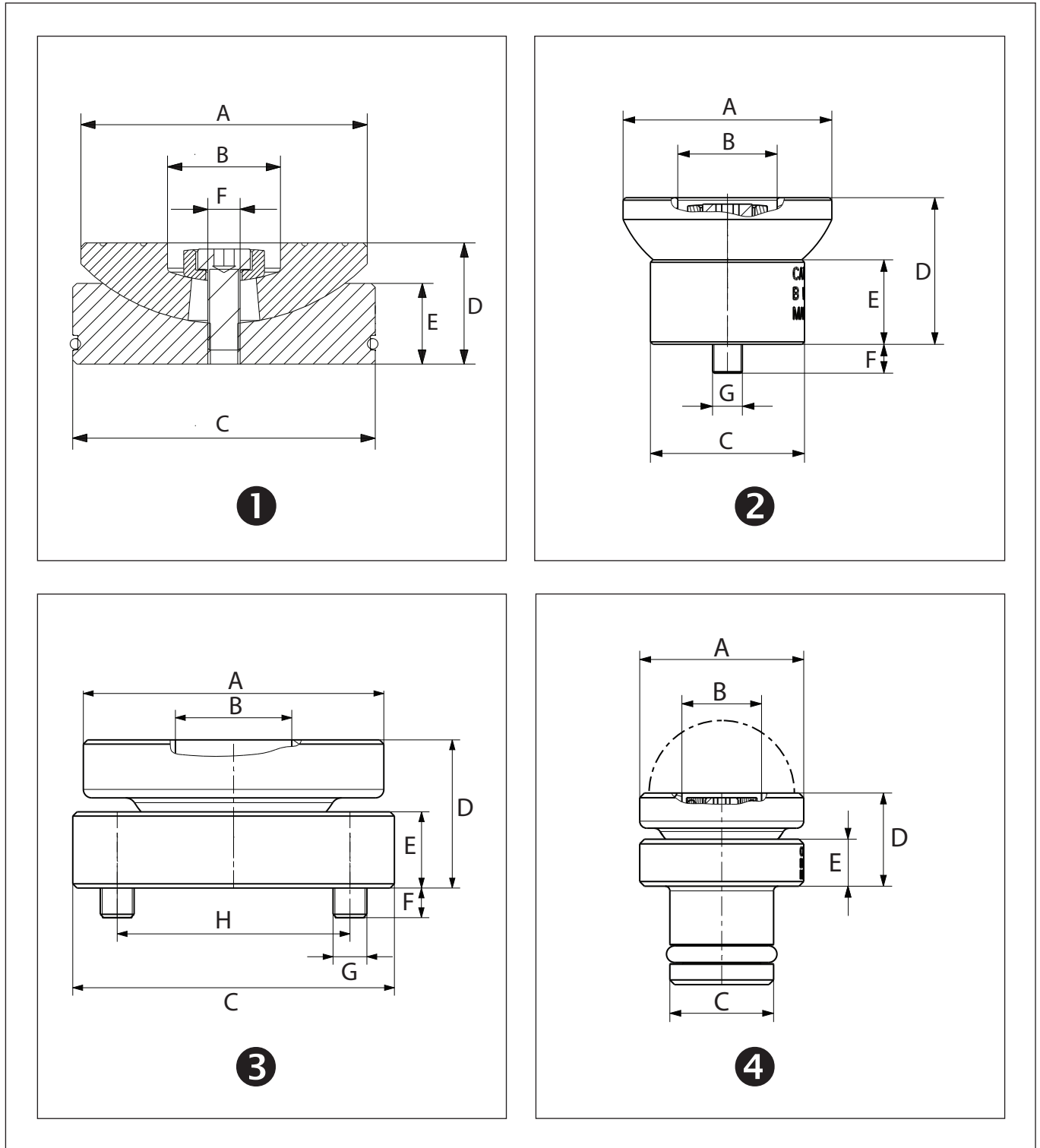
Figure 2: Tilt saddle dimensions
