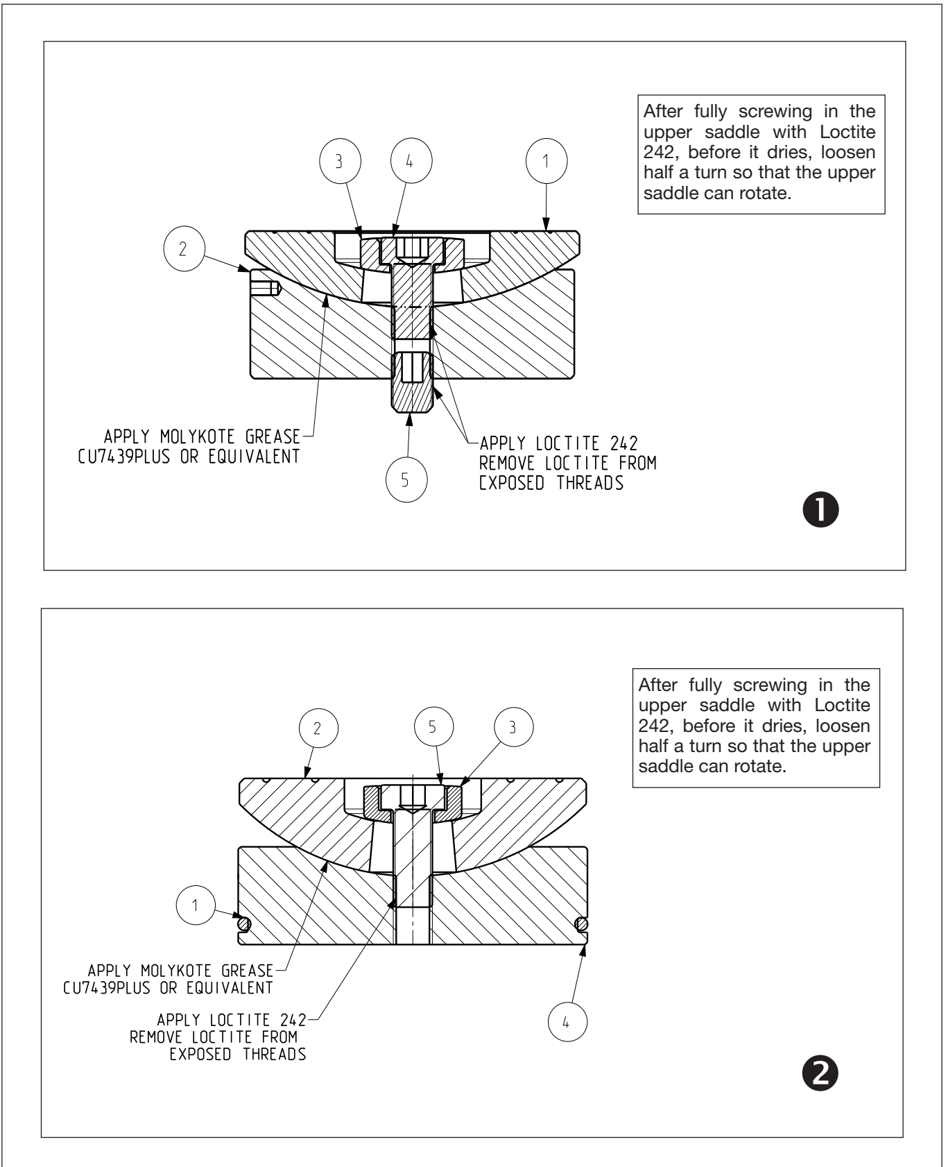
Figure 4: Tilt Saddles Internal View
