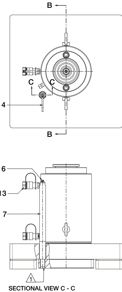
Fig. 1, Main Assembly
