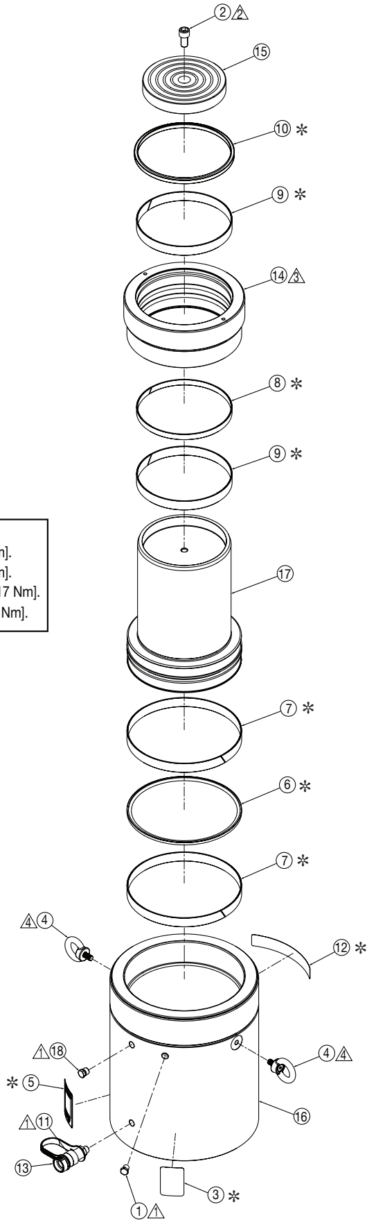
Figure 4, Exploded View - Model HCG-400
