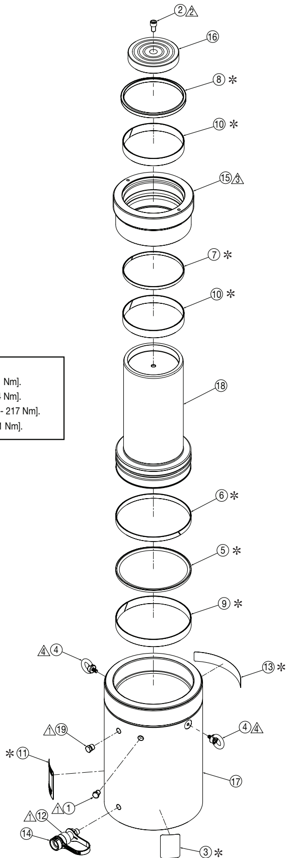
Figure 2, Exploded View - Model HCG-250 Tall
