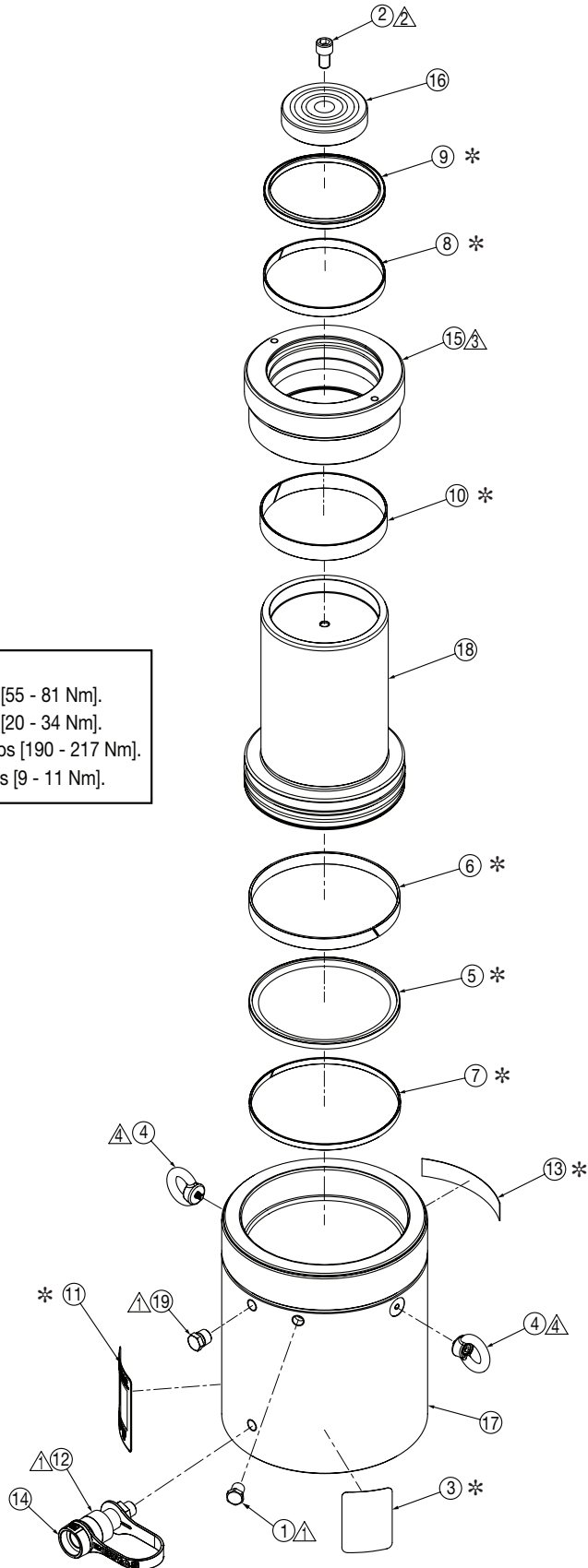
Figure 1, Exploded View - Model HCG-250 Short
