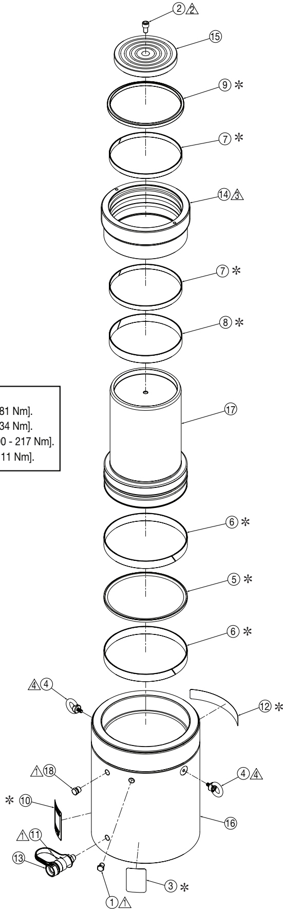
Figure 3, Exploded View - Model HCG-300
