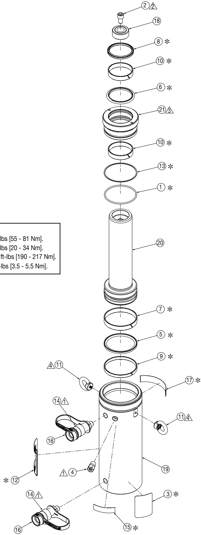
Figure 2, Exploded View - Model HCR-50 Tail
