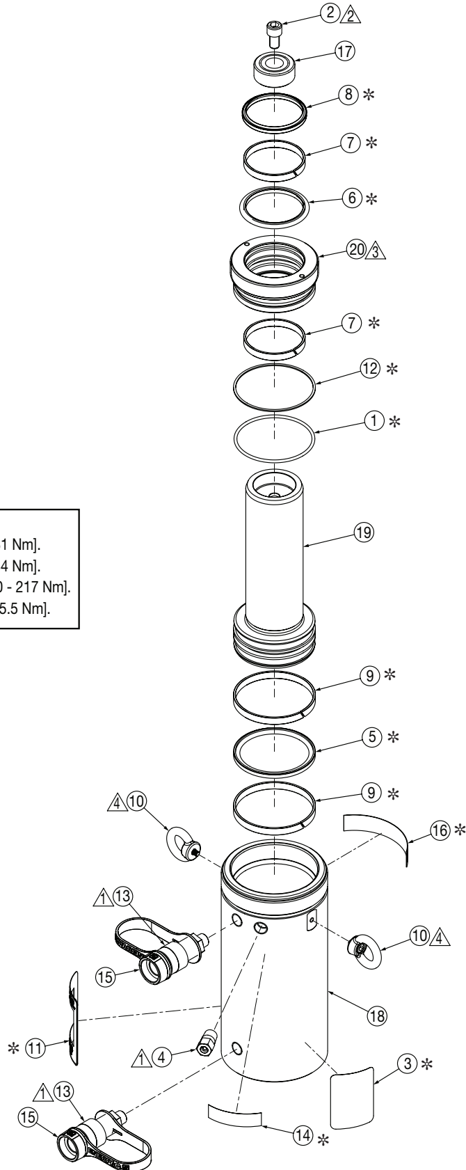
Figure 1, Exploded View - Model HCR-50 Short
