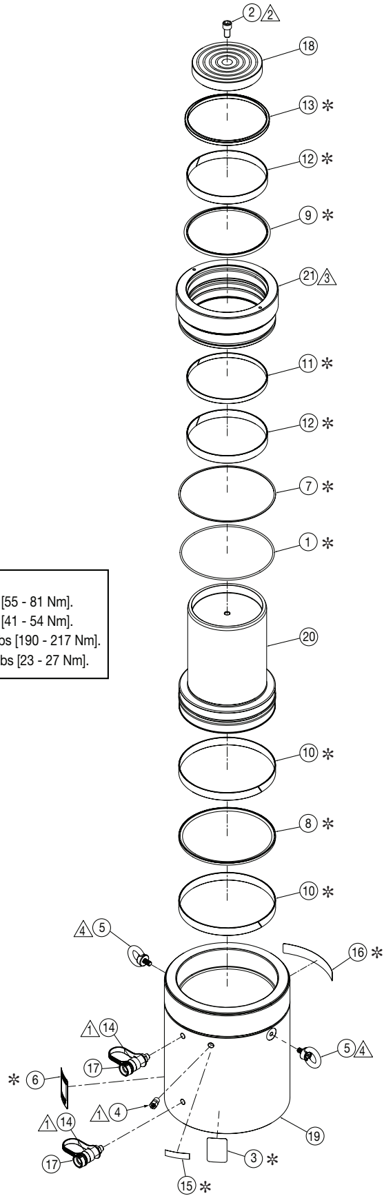
Figure 4, Exploded View - Model HCR-400
