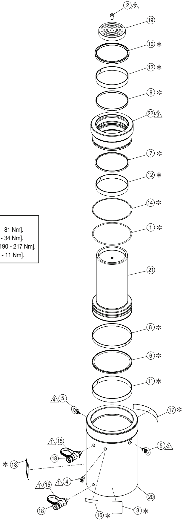
Figure 2, Exploded View - Model HCR-250 Tall
