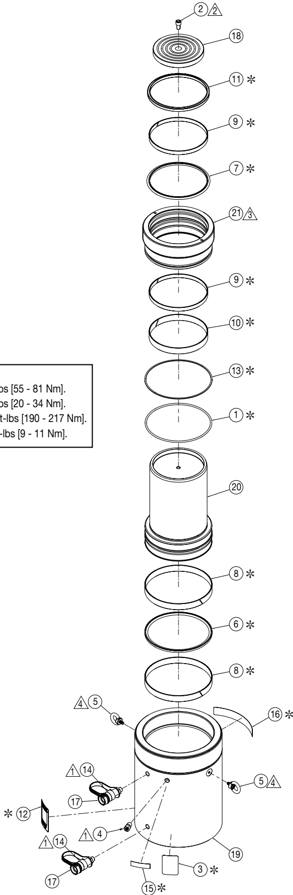
Figure 3, Exploded View - Model HCR-300
