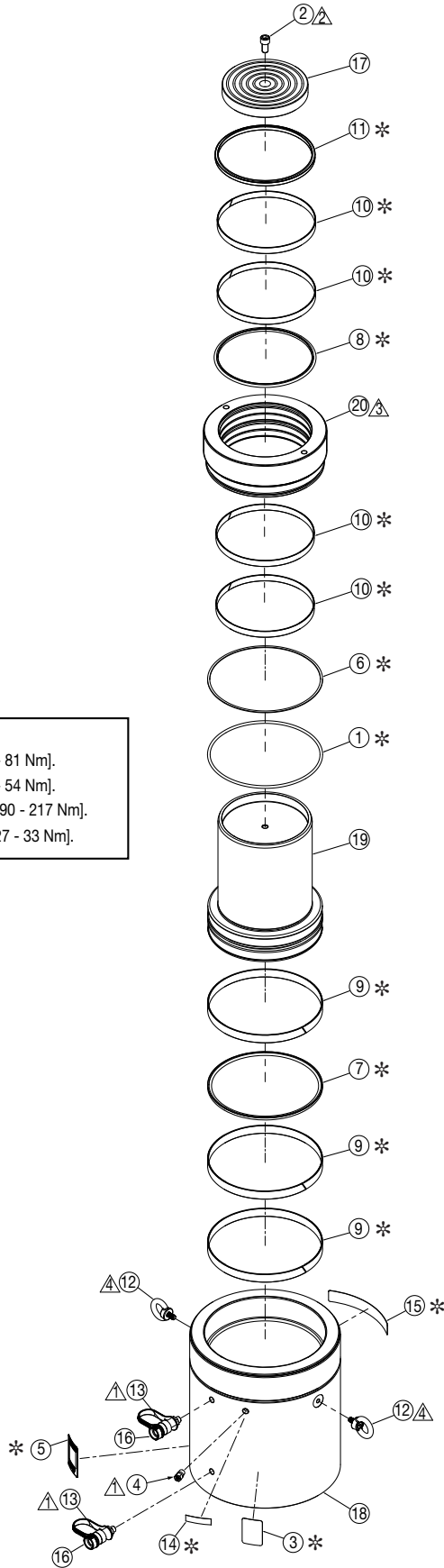
Figure 4, Exploded View - Model HCR-1000
