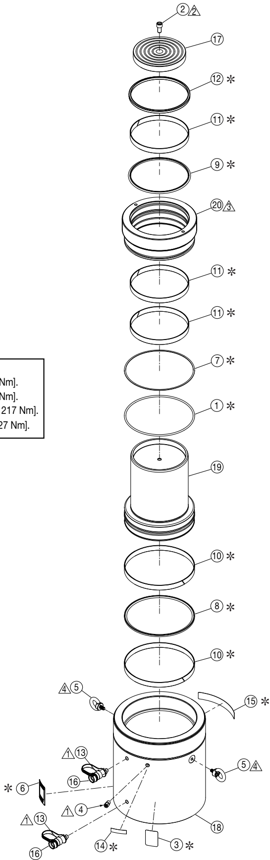
Figure 2, Exploded View - Model HCR-600
