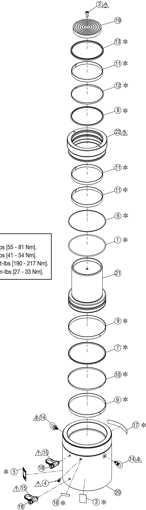
Figure 3, Exploded View - Model HCR-800
