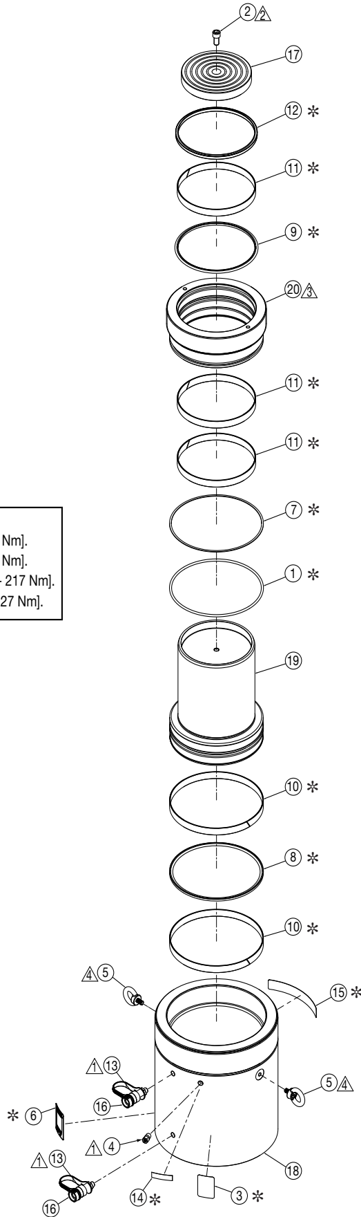
Figure 1, Exploded View - Model HCR-500
