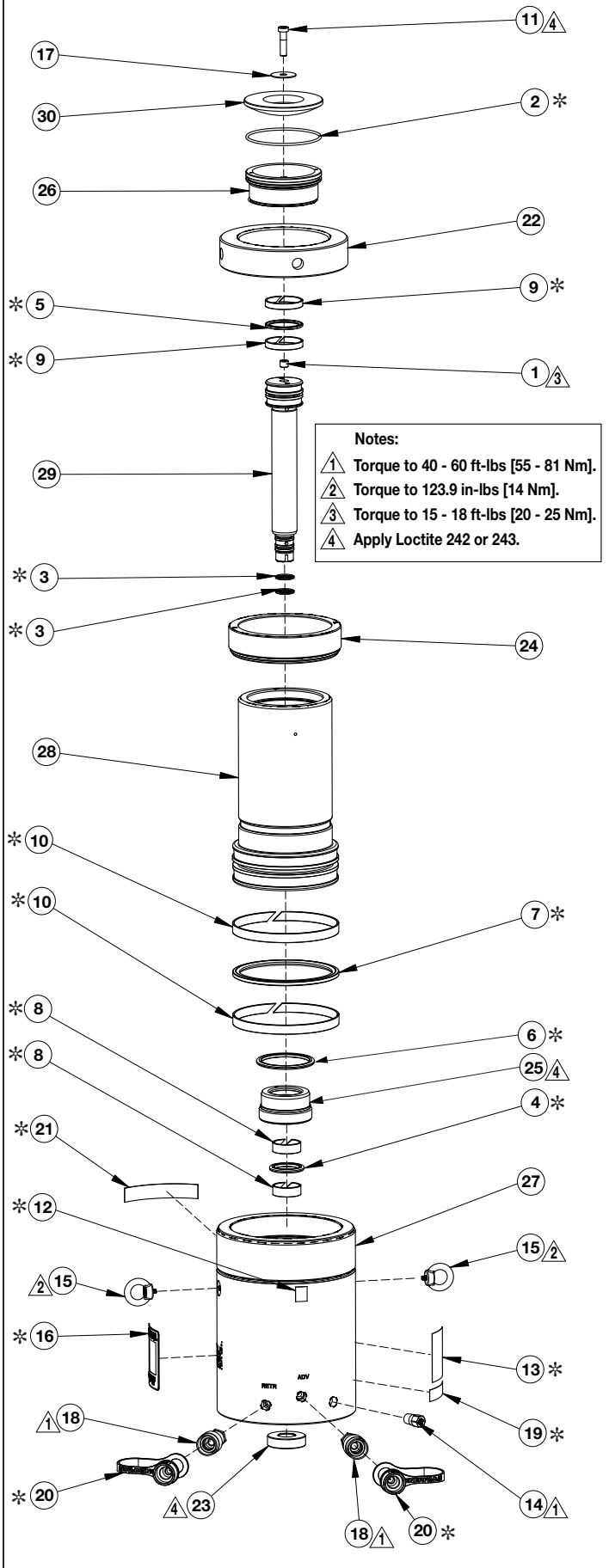
Figure 1, Exploded View - Model HCRL 1502-1506
