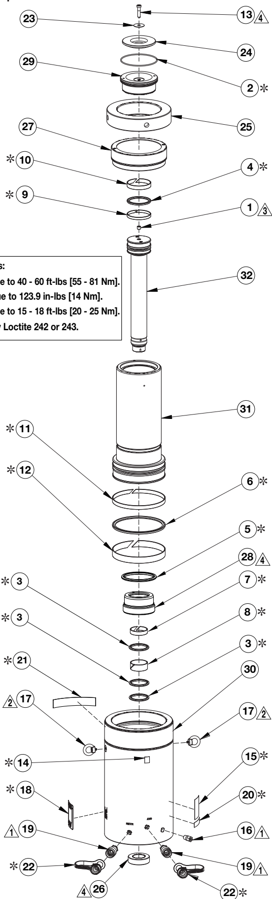
Figure 2, Exploded View - Model HCRL 2008-2012
