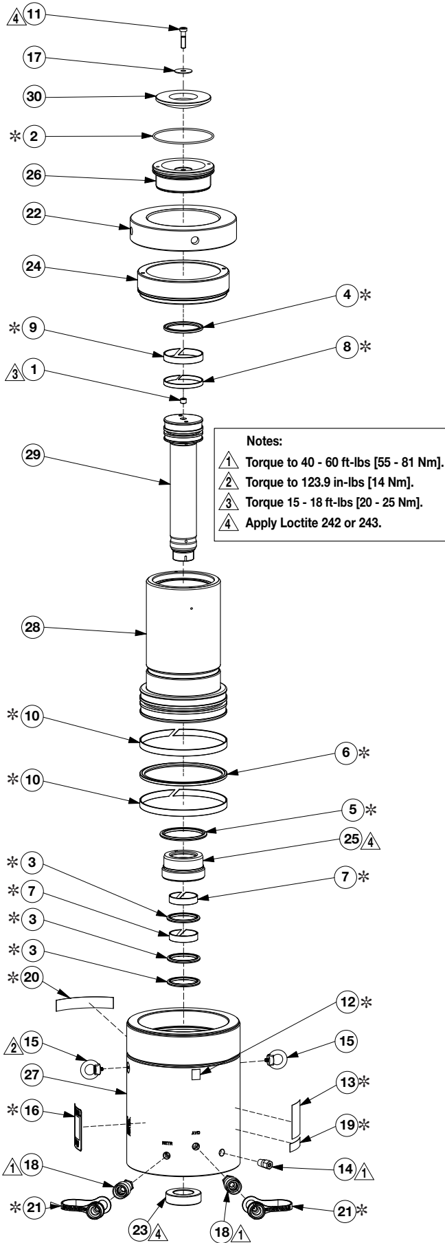
Figure 1, Exploded View - Model HCRL 2002-2006
