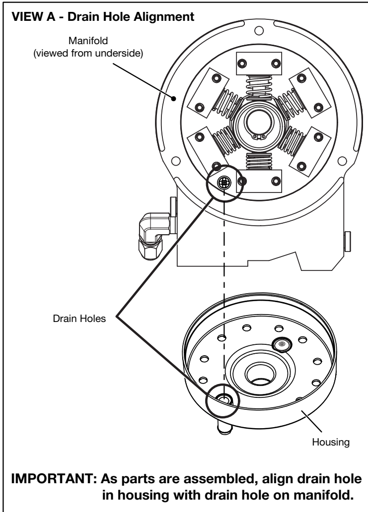
Figure 6, Motor Replacement Kit
