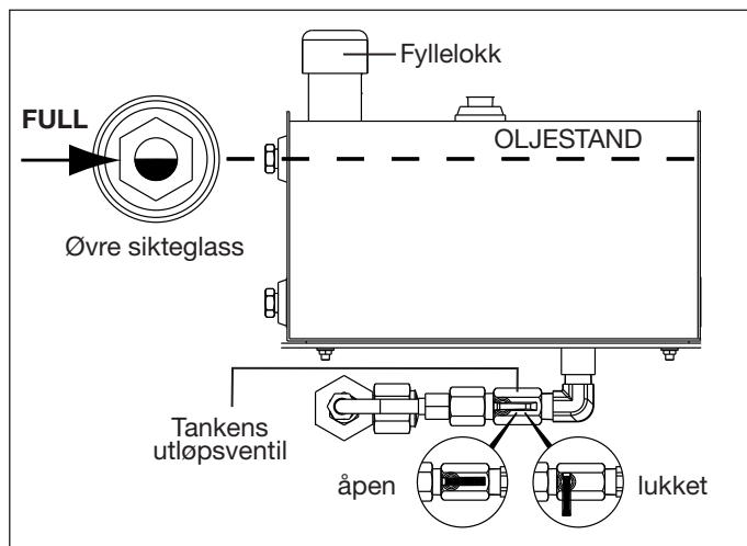
Figur 3, Hydraulikkoljetank
