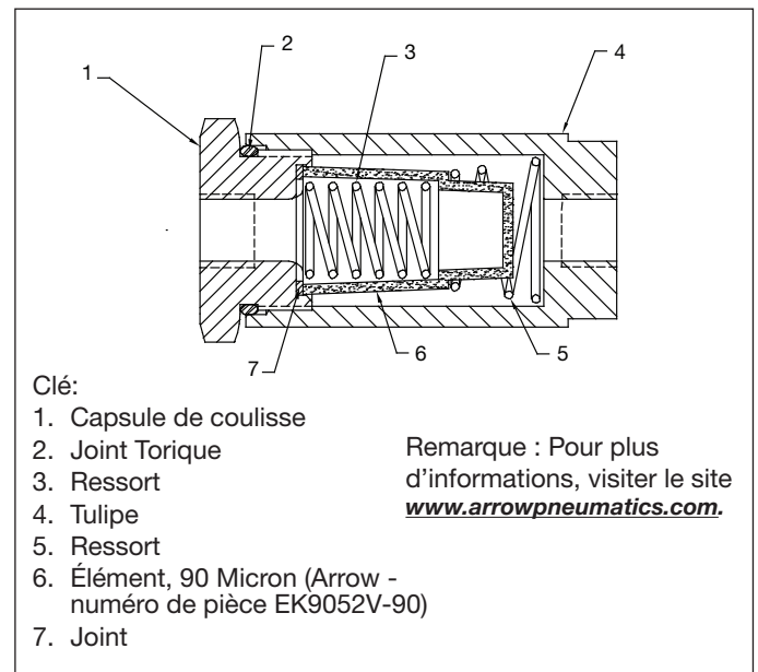
Figure 11, Hydraulic Filter Details
