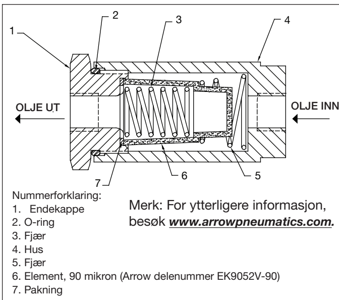
Figur 11, Detaljer, hydraulikkfilter
