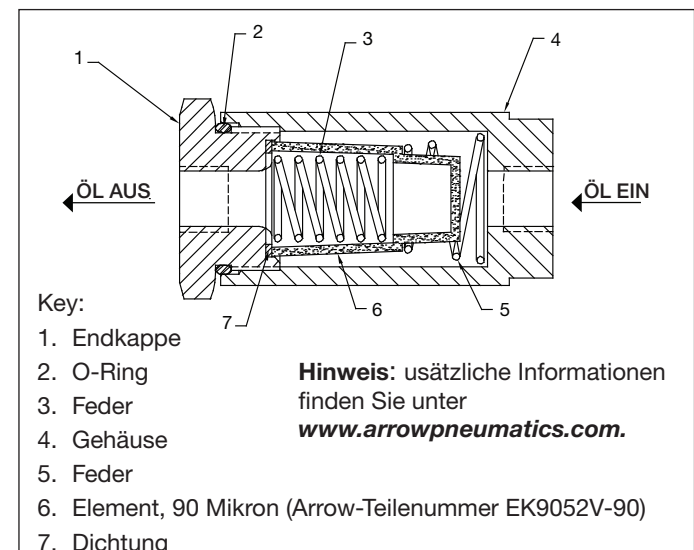
Abb. 11, Hydraulikfilter-Details
