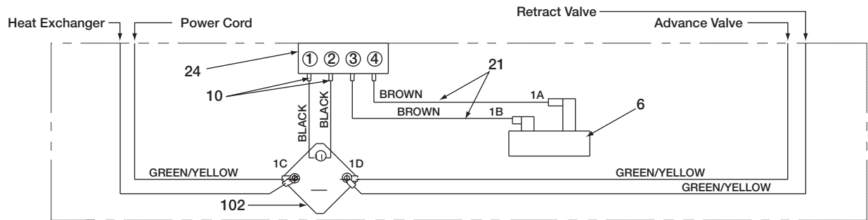
Figure 8, Wiring Diagram
