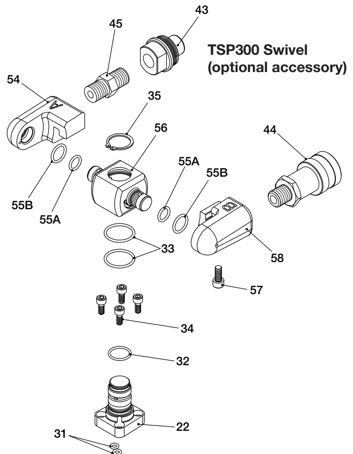
Figure 2, Swivel Assemblies, Model S11000X
