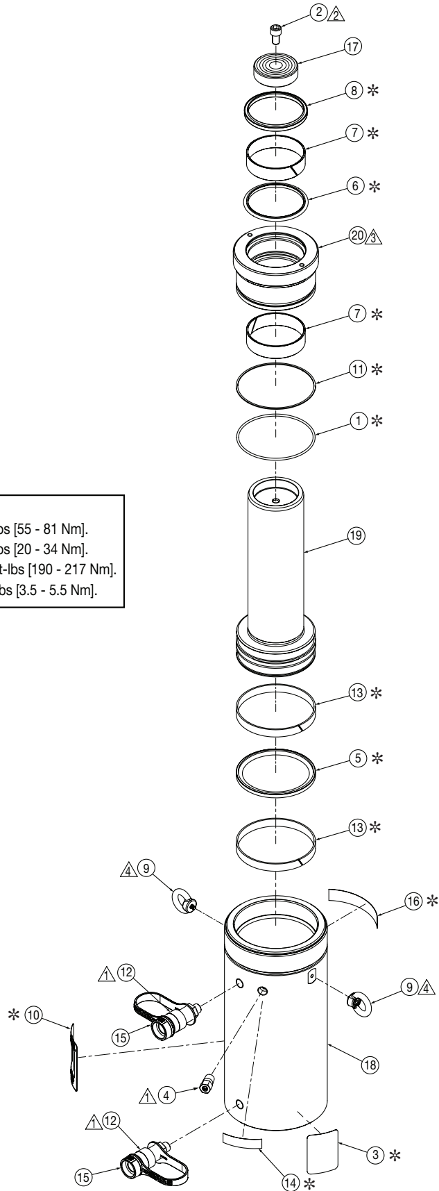
Figure 4, Exploded View - Model HCR-100 Tall
