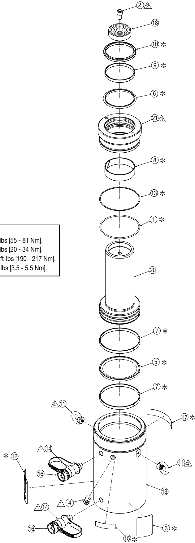
Figure 3, Exploded View - Model HCR-100 Short
