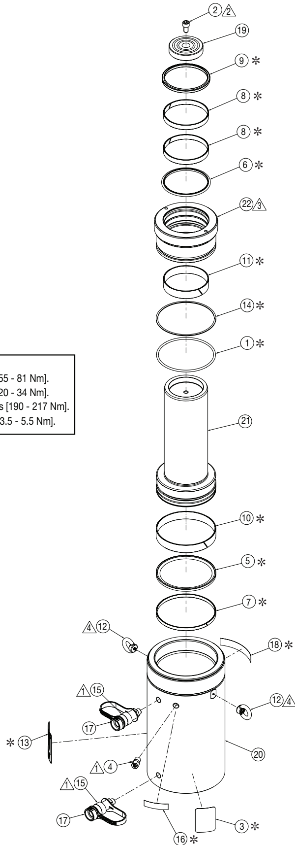
Figure 2, Exploded View - Model HCR-150 Tall
