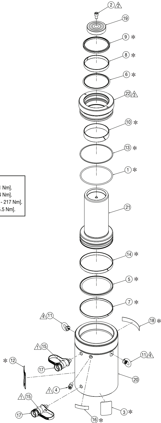
Figure 1, Exploded View - Model HCR-150 Short
