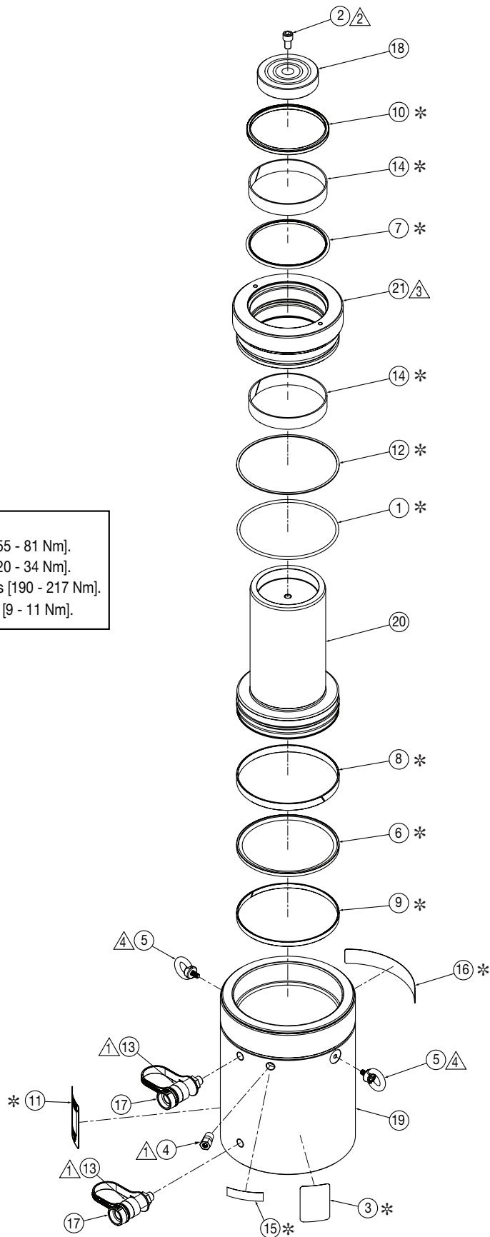
Figure 3, Exploded View - Model HCR-200 Short
