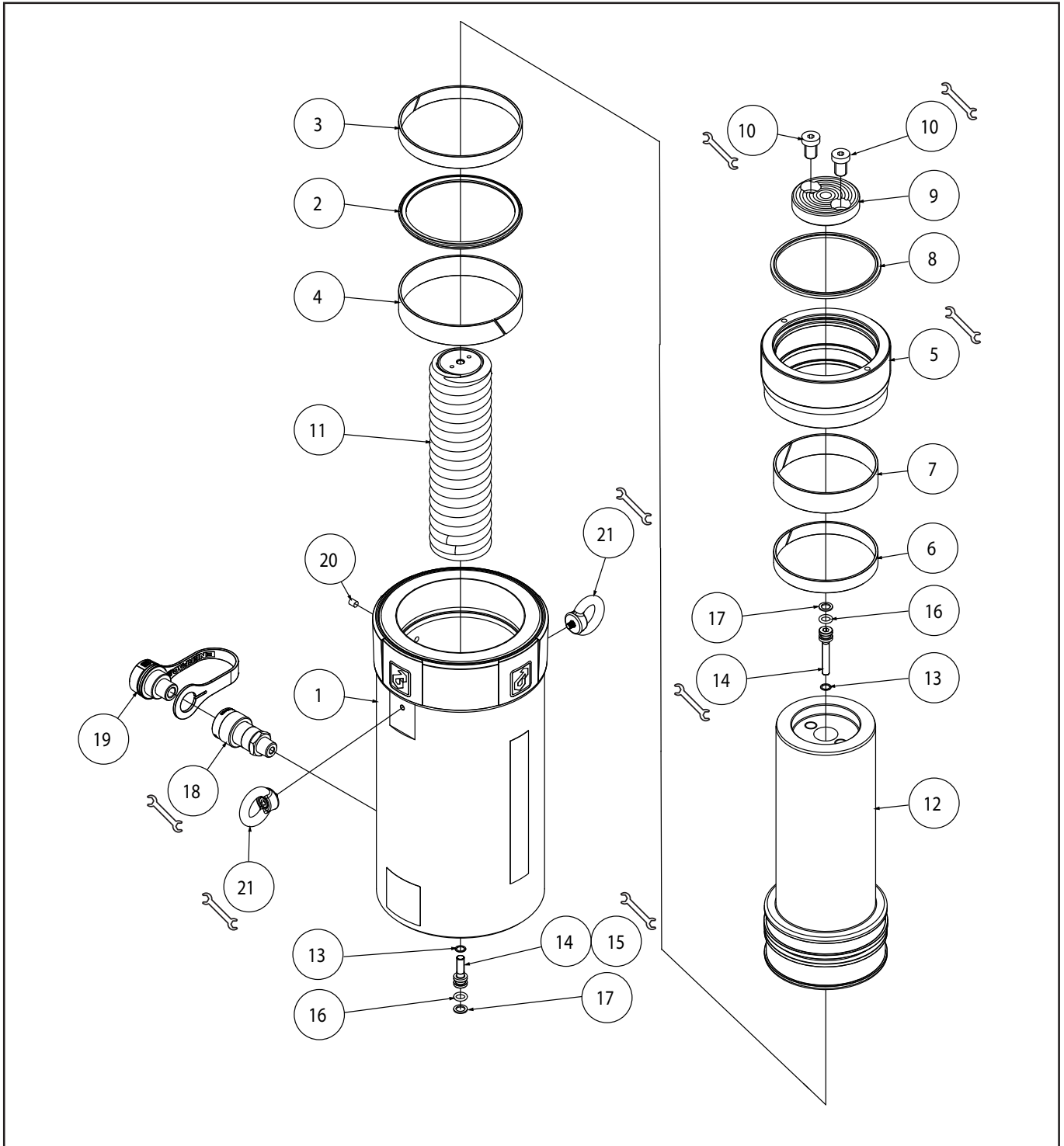
Figure 1, RC Hydraulic Cylinder, 100 Ton
