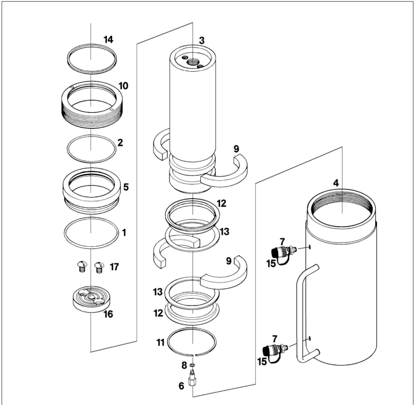
75 Ton 6" Stroke Double-Acting Hydraulic Cylinder
